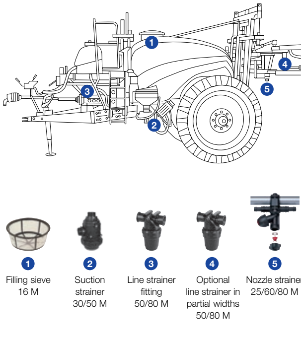
Scheme for selecting the mesh size using the example of a field sprayer:
