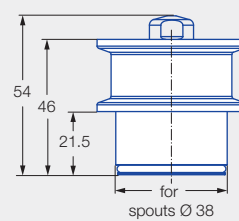
Tri-Clamp connection
