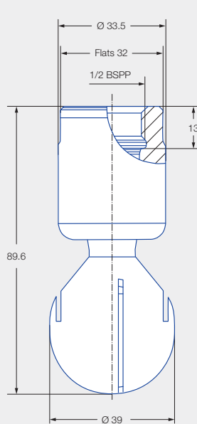
Female thread
