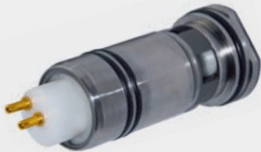
EVA quick connect 52 mm/2" with offset pins
