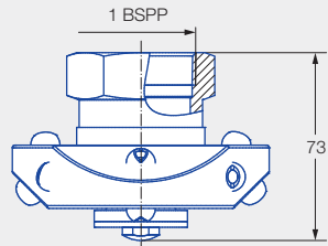
Female thread
