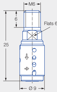
Male thread
