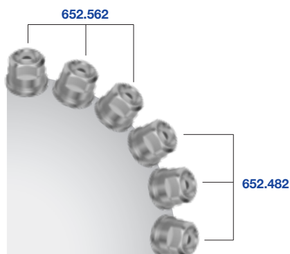
Example equipment (one-side) of an axial blower with flat jet nozzles 30°.
